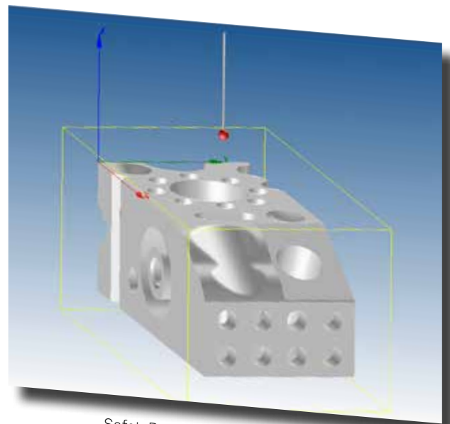
SafetyBox for collision-free probing
