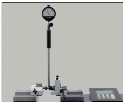
Setting of 2-point bore gauges (TEL5/TA-SU-301)
