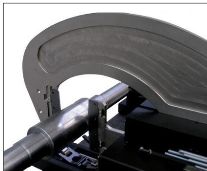
Installation for eccentric diameter measurement (specific design)
